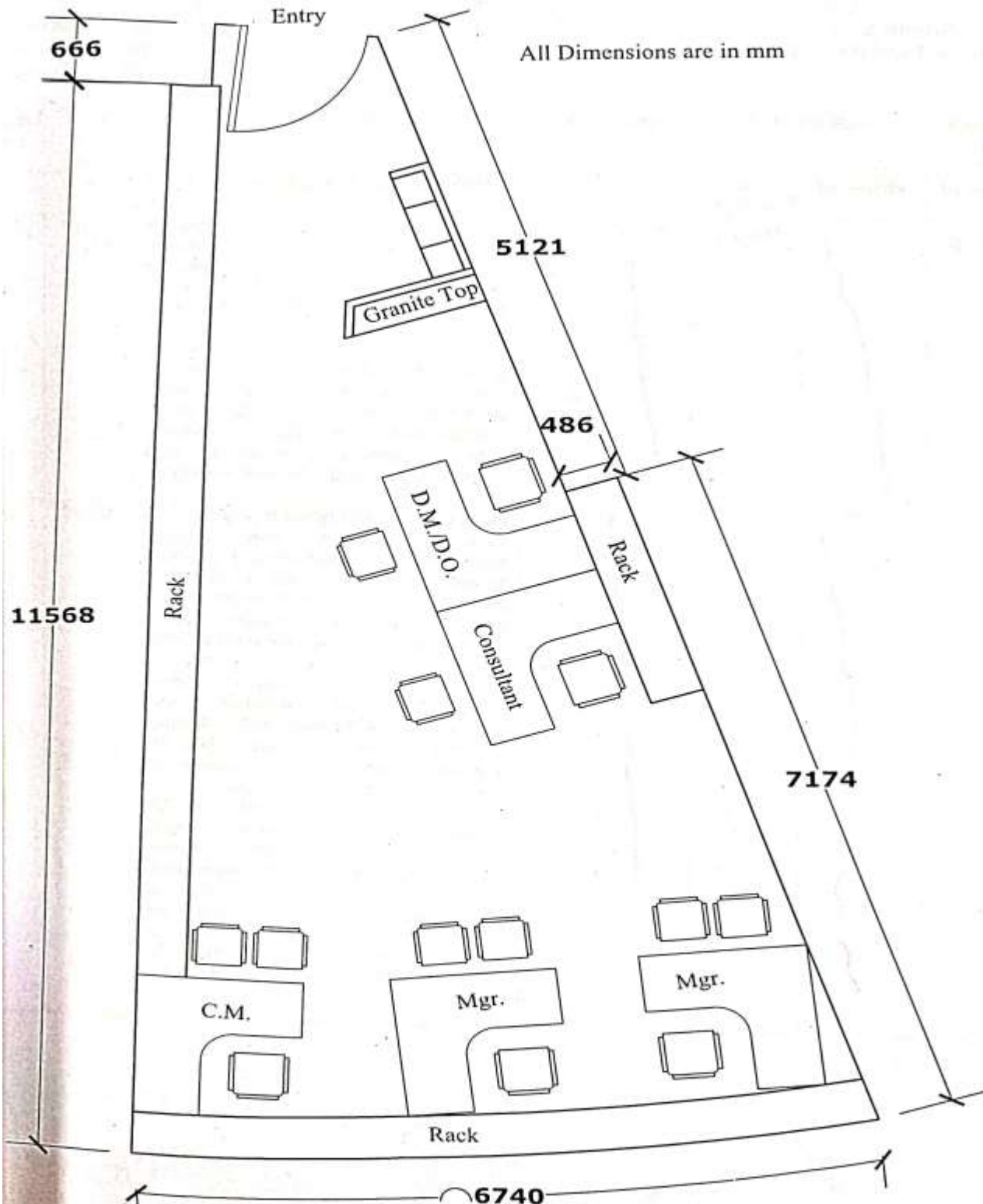
Proposed Layout Plan for setting up of NSIC-MDBP Project Office In the Existing module No. 13 B
