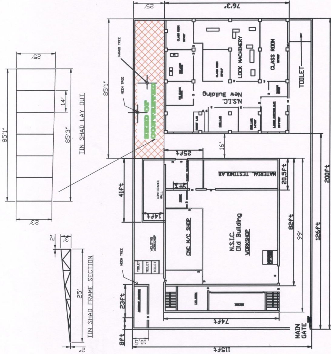
LAY OUT OF N.S.I.C BUILDING (GROUND FLOOR)
