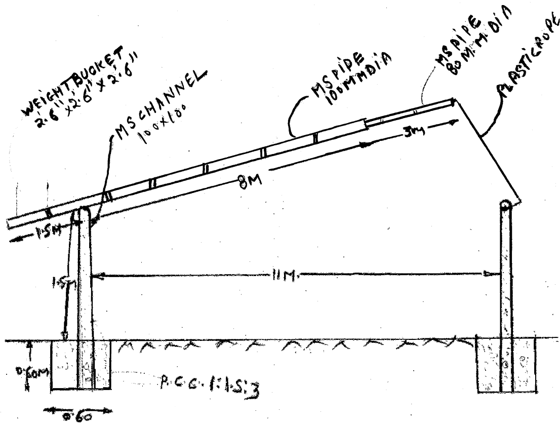
Schematic Drawing of Barrier.
